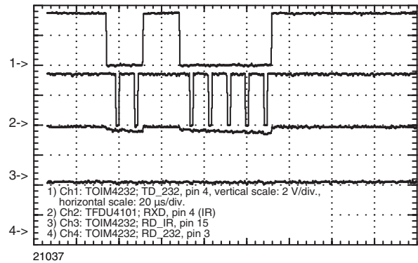
Figure 14. Echo-Suppression
